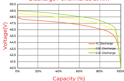
Discharge Performance at R.T.
